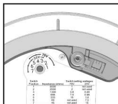
Transformer adjustment from rear (under rubber plug).
