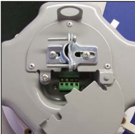
Rear entry plate with included squeeze connector.
