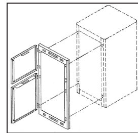
SECURE: A bracket keeps contents in bottom space secure when top door is open (bracket projects into rack within 1/4" of mounting rails). Two machine screws are provided for field installation (8-32 x .5"). Factory installed when frame, doors, and rack are ordered together.
