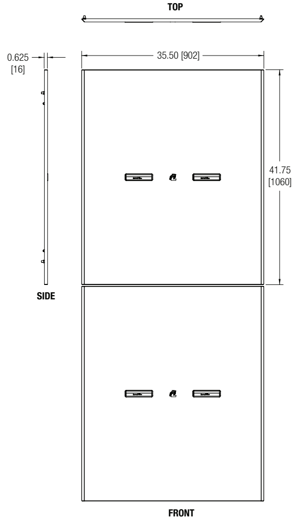
Model SDPN-4536 (2pcs, per side)
