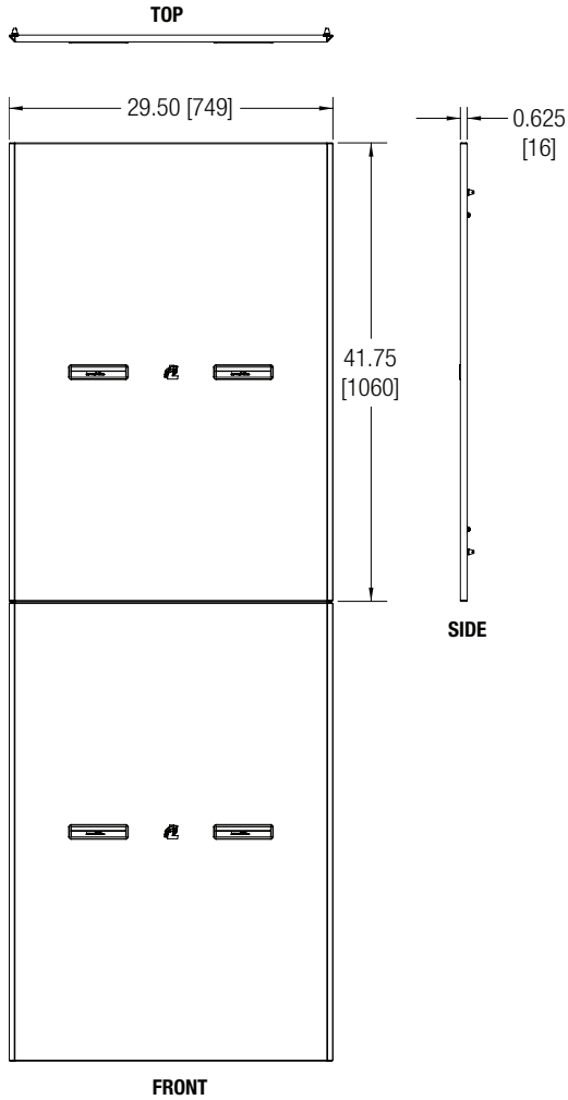
Model SDPN-4530 (2pcs, per side)
