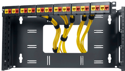
Front hinge swings out 180 degrees (left or right, depending on how it's mounted)
