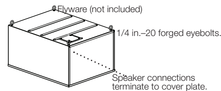
Fig. 2: Suspended into Rigid or Tile Ceiling
