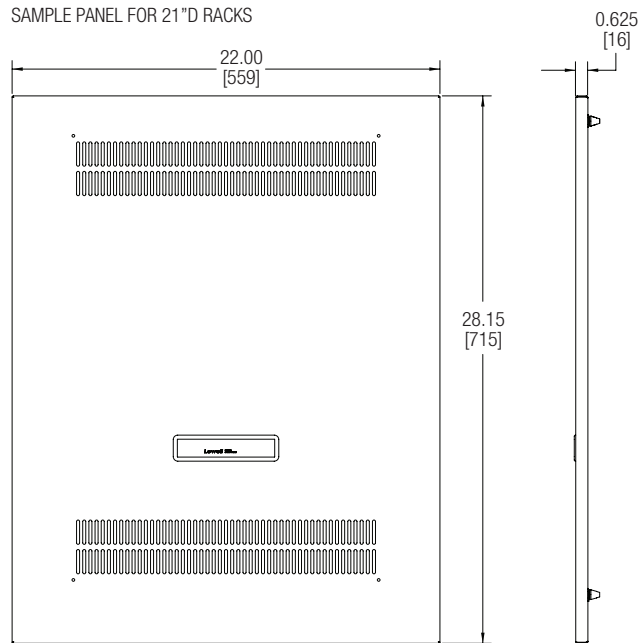
SAMPLE PANEL FOR 21"D RACKS
