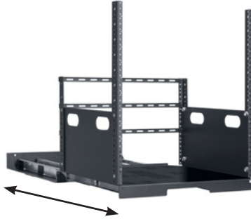
Rack slides forward for access to the rear of equipment and connections.
