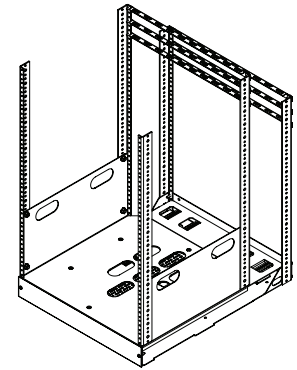
ISO VIEW
