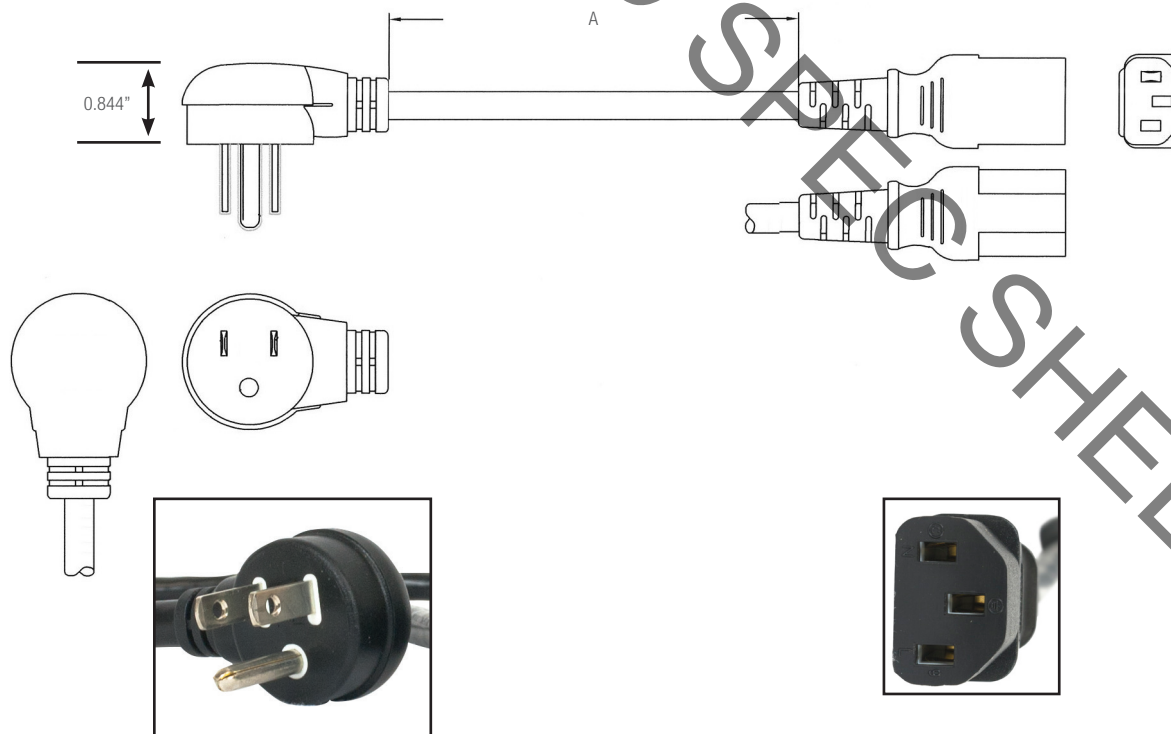
Cord with low-profile left-angled / right-angled plug
